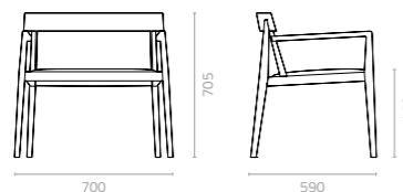
Astras arm lounge chair W700 x D590 x H705 x SH410mm Packing: 0.313m 3 , 1pc/ctn
