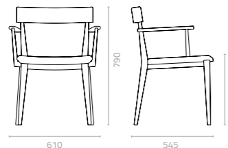
Country I arm chair W610 x D545 x H790 x SH450mm Packing: 0.330m 3 , 1pc/ctn
