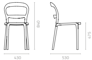
Heather chair with Artwood seat W430 x D530 x H840 x SH475mm Packing: 0.288m 3 , 4pcs/ctn Stackable
