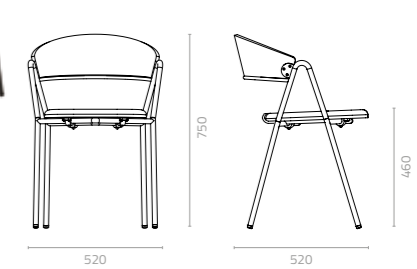
Latte chair W520 x D520 x H750 x SH460mm Packing: 0.253m 3 , 2pcs/ctn
