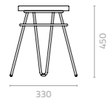
Hairpin stool with rubberwood seat W330 x D330 x H450mm Packing: 0.060m 3 , 1pc/ctn
