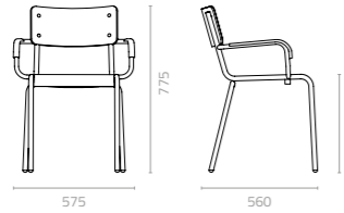
Agape arm chair W575 x D560 x H775 x SH460mm Packing: 0.365m 3 , 4pcs/ctn Stackable
