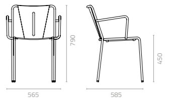
Inicio-V arm chair with bentwood seat W565 x D585 x H790 x SH450mm Packing: 0.346m 3 , 4pcs/ctn Stackable
