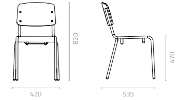
Barry chair W420 x D535 x H820 x SH470mm Packing: 0.244m 3 , 4pcs/ctn Stackable
