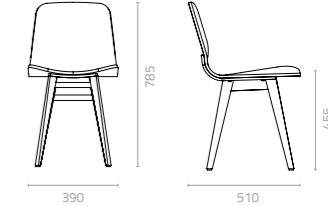
Kay chair with wooden base W390 x D510 x H785 x SH455mm Packing: 0.263m 3 , 2pcs/ctn
