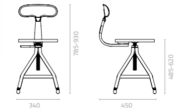
New York chair (adjustable seat height) W340 x D450 x H785-930 x SH485-620mm Packing: 0.140m 3 , 1pc/ctn Swivel
