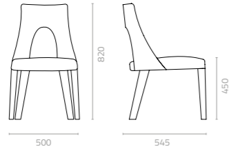
Ópera lite chair W500 x D545 x H820 x SH450mm Packing: 0.421m 3 , 2pcs/ctn
