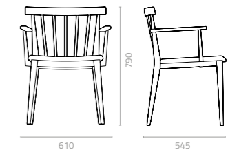
Country IV arm chair W610 x D545 x H790 x SH450mm Packing: 0.330m 3 , 1pc/ctn
