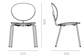
Ovni chair W520 x D530 x H800 x SH450mm Packing: 0.289m 3 , 4pcs/ctn Stackable
