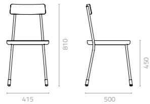
Lara chair W415 x D500 x H810 x SH450mm Packing: 0.201m 3 , 4pcs/ctn
