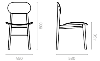
Dana chair W450 x D530 x H800 x SH450mm Packing: 0.287m 3 , 2pcs/ctn
