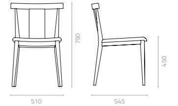
Country II chair W510 x D545 x H790 x SH450mm Packing: 0.327m 3 , 2pcs/ctn
