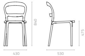
Heather chair with wicker seat W430 x D530 x H840 x SH475mm Packing: 0.288m 3 , 4pcs/ctn Stackable
