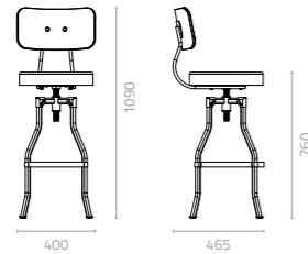
Markenzi barstool (fixed height) W400 x D465 x H1090 x SH760mm Packing: 0.196m 3 , 1pc/ctn
