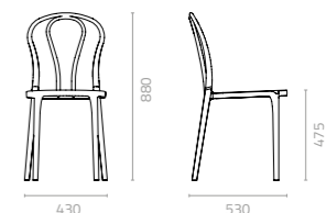
Parker chair with PP seat W430 x D530 x H880 x SH475mm Packing: 0.274m 3 , 4pcs/ctn Stackable
