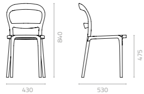
Heather chair with PP seat W430 x D530 x H840 x SH475mm Packing: 0.288m 3 , 4pcs/ctn Stackable
