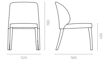
Blow chair W520 x D585 x H780 x SH450mm Packing: 0.469m 3 , 2pcs/ctn Stackable
