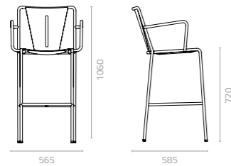
Inicio-V arm barstool W565 x D585 x H1060 x SH720mm Packing: 0.457m 3 , 4pcs/ctn
