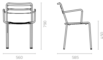
Inicio arm chair W560 x D585 x H790 x SH450mm Packing: 0.337m 3 , 4pcs/ctn Stackable
