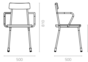
Lara arm chair W500 x D500 x H810 x SH450mm Packing: 0.289m 3 , 4pcs/ctn
