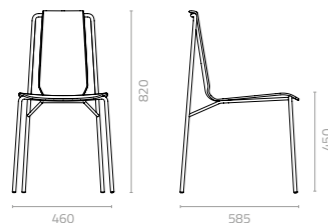
Achilla chair W460 x D585 x H820 x SH450mm Packing: 0.312m 3 , 4pcs/ctn Stackable
