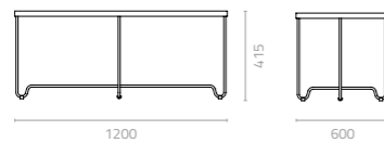
Matrix rectangular W1200 x D600 x H415 Packing: 0.406m 3 , 2stacks/set
