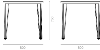
Hairpin II dining table W800 x D800 x H750mm Packing: 0.070m 3 , 1set/2ctns Custom sizes available
