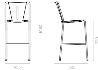
Inicio-V barstool W455 x D585 x H1060 x SH720mm Packing: 0.329m 3 , 4pcs/ctn
