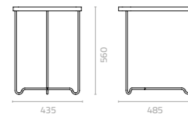
Matrix triangle coffee table W435 x D485 x H560 Packing: 0.154m 3 , 2ctns/set
