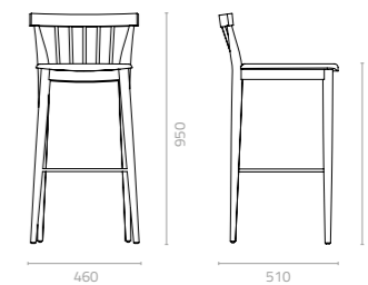
Country IV barstool W460 x D510 x H950 x SH750mm Packing: 0.240m 3 , 1pc/ctn
