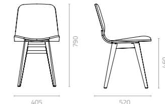
Kay chair shell upholstery with wooden base W405 x D520 x H790 x SH460mm Packing: 0.263m 3 , 2pcs/ctn
