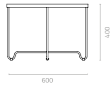
Matrix round coffee table Ø600 x H400 Packing: 0.184m 3 , 2ctns/set
