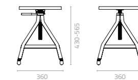
New York low stool (adjustable seat height) W360 x D360 x H430-565mm Packing: 0.063m 3 , 1pc/ctn Swivel
