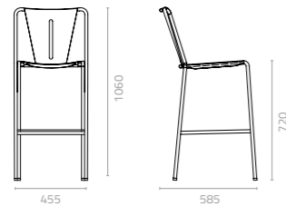
Inicio-V barstool with bentwood seat W455 x D585 x H1060 x SH720mm Packing: 0.329m 3 , 4pcs/ctn
