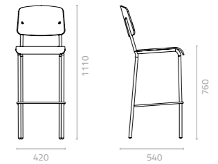
Barry barstool W420 x D540 x H1110 x SH760mm Packing: 0.244m 3 , 1pc/ctn
