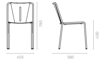
Inicio-V chair with bentwood seat W455 x D585 x H790 x SH450mm Packing: 0.241m 3 , 4pcs/ctn Stackable
