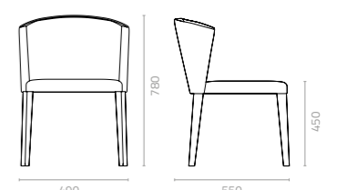
Cady chair W490 x D550 x H780 x SH450mm Packing: 0.464m 3 , 2pcs/ctn Stackable
