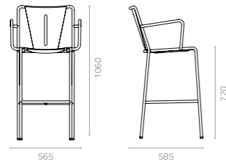
Inicio-V arm barstool with bentwood seat W565 x D585 x H1060 x SH720mm Packing: 0.457m 3 , 4pcs/ctn
