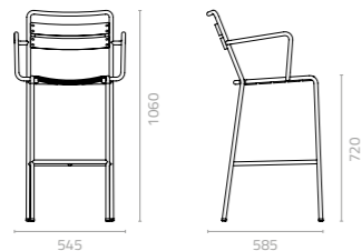
Inicio arm barstool W545 x D585 x H1060 x SH720mm Packing: 0.446m 3 , 4pcs/ctn
