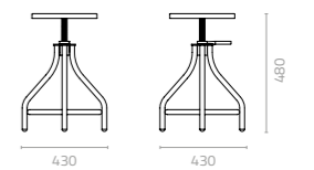
Inicio bistro stool (fixed height) W430 x D430 x H480mm Packing: 0.095m 3 , 1pc/ctn
