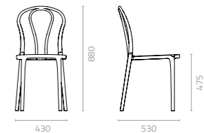
Parker chair with Artwood seat W430 x D530 x H880 x SH475mm Packing: 0.274m 3 , 4pcs/ctn Stackable
