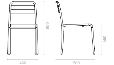
Bart chair W460 x D580 x H800 x SH460mm Packing: 0.340m 3 , 4pcs/ctn Stackable
