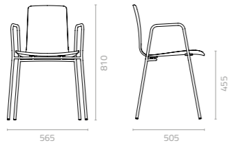
Zeat arm chair W565 x D505 x H810 x SH455mm Packing: 0.425m 3 , 4pcs/ctn Stackable
