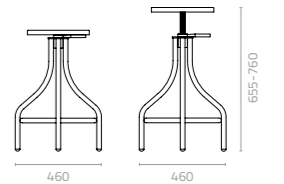
Inicio bistro adjustable highstool with metal seat W460 x D460 x H655-760mm Packing: 0.120m 3 , 1pc/ctn Swivel
