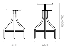
Inicio bistro adjustable highstool with rubberwood seat W460 x D460 x H655-760mm Packing: 0.126m 3 , 1pc/ctn Swivel
