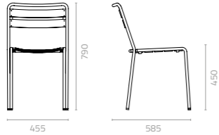
Inicio chair W455 x D585 x H790 x SH450mm Packing: 0.232m 3 , 4pcs/ctn Stackable
