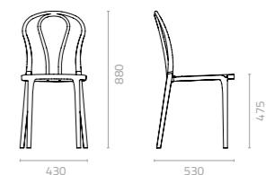
Parker chair with textylene seat W430 x D530 x H880 x SH475mm Packing: 0.274m 3 , 4pcs/ctn Stackable
