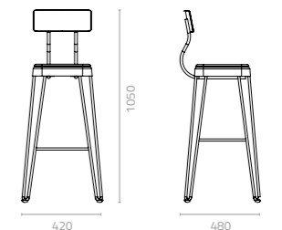
Kaemi barstool with upholstered seat W420 x D480 x H1050 x SH750mm Packing: 0.177m 3 , 1pc/ctn
