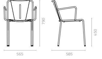
Inicio-V arm chair W565 x D585 x H790 x SH450mm Packing: 0.337m 3 , 4pcs/ctn Stackable
