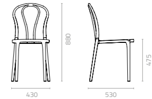
Parker chair with wicker seat W430 x D530 x H880 x SH475mm Packing: 0.274m 3 , 4pcs/ctn Stackable
