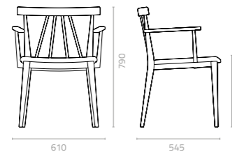
Country III arm chair W610 x D545 x H790 x SH450mm Packing: 0.330m 3 , 1pc/ctn
