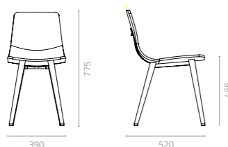
Taco chair W390 x D520 x H775 x SH455mm Packing: 0.263m 3 , 2pcs/ctn
