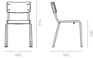
Agape chair W485 x D560 x H775 x SH460mm Packing: 0.273m 3 , 4pcs/ctn Stackable
