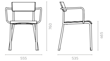
T-arm chair - plywood W555 x D535 x H760 x SH465mm Packing: 0.365m 3 , 4pcs/ctn Stackable
