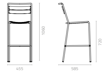
Inicio barstool W455 x D585 x H1060 x SH720mm Packing: 0.319m 3 , 4pcs/ctn
