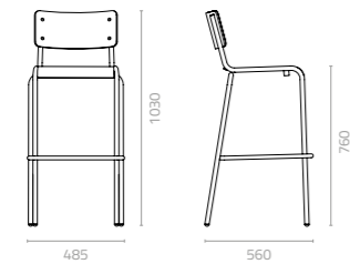
Agape barstool W485 x D560 x H1030 x SH760mm Packing: 0.365m 3 , 4pcs/ctn Stackable
