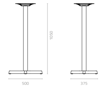
Barkas bartable Base W500 x D375 x H1050
