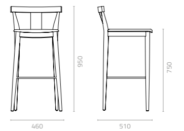
Country II barstool W460 x D510 x H950 x SH750mm Packing: 0.240m 3 , 1pc/ctn
