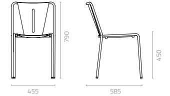
Inicio-V chair W455 x D585 x H790 x SH450mm Packing: 0.232m 3 , 4pcs/ctn Stackable
