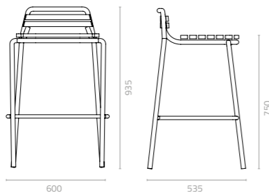
Adela barstool W600 x D535 x H935 x SH750mm Packing: 0.398m 3 , 2pcs/ctn Stackable
