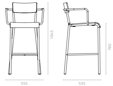
T-arm barstool - plywood W555 x D535 x H1045 x SH760mm Packing: 0.488m 3 , 4pcs/ctn
