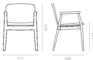
Grado arm chair W575 x D560 x H820 x SH450mm Packing: 0.296m 3 , 1pc/ctn
