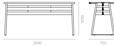
Skyler bar table W2000 x D750 x H1050mm Packing: 1.302m 3 , 1set/3ctns
