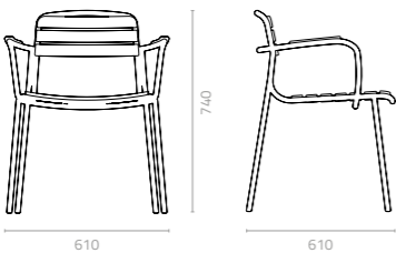
Adela arm chair W610 x D610 x H740mm Packing: 0.650m 3 , 4pcs/ctn Stackable
