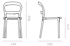
Heather chair with textylene seat W430 x D530 x H840 x SH475mm Packing: 0.288m 3 , 4pcs/ctn Stackable
