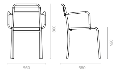
Bart arm chair W560 x D580 x H800 x SH460mm Packing: 0.400m 3 , 4pcs/ctn Stackable
