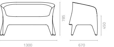
Obie love seat W1300 x D670 x H785 x SH450mm Packing: 0.770m 3 , 1pc/ctn
