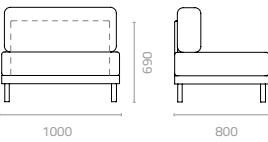
TCB centre W1000 x D800 x H690 x SH400mm Packing: 0.616m 3 , 1pc/stack
