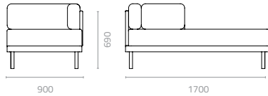
TCB lounge (right) W900 x D1700 x H690 x SH400mm Packing: 1.158m 3 , 1pc/stack
