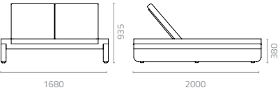
Attitude double sunbed W1680 x D2000 x H935 x SH380mm Packing: 1.170m 3 , 1pc/ctn
