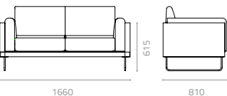
Moel 2-seater sofa W1660 x D810 x H615 x SH400mm Packing: 0.916m 3 , 1pc/stack
