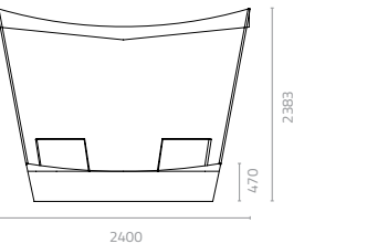
Dream dot day bed W2400 x D2400 x H2383 x SH470mm Packing: 2.700m 3 , 1pcs/stack
