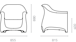
Pinch 1-seater sofa W855 x D815 x H880 x SH400mm Packing: 0.640m 3 , 1pc/ctn
