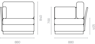
Mediterranean corner sofa W880 x D880 x H840 x SH405mm Packing: 0.605m 3 , 1pc/ctn
