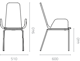
Olivia arm chair W510 x D600 x H940 x SH440mm Packing: 0.320m 3 , 1pc/stack
