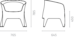
Obie arm chair W765 x D645 x H785 x SH450mm Packing: 0.430m 3 , 1pc/ctn
