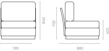
Mediterranean centre sofa W785 x D880 x H840 x SH405mm Packing: 0.541m 3 , 1pc/ctn
