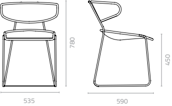
Basket chair W535 x D590 x H780 x SH450mm Packing: 0.290m 3 , 1pc/ctn
