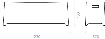
Rumble bench W1230 x D370 x H450mm Packing: 0.200m 3 , 1pc/ctn
