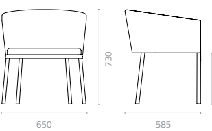
Chameleon 4L chair W650 x D585 x H730 x SH445mm Packing: 0.350m 3 , 1pc/ctn
