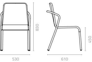
Flap chair (full weaving) W530 x D610 x H830 x SH450mm Packing: 0.450m 3 , 4pcs/ctn Stackable
