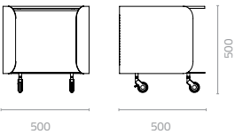
Vienna side table Ø500 x H500mm Packing: 0.166m 3 , 2ctn/set
