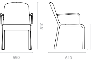
Rango arm chair (full weaving) W550 x D610 x H810 x SH455mm Packing: 0.450m 3 , 4pcs/stack Stackable
