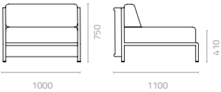
Sky centre unit W1000 x D1100 x H750 x SH410mm Packing: 1.050m 3 , 1pc/ctn
