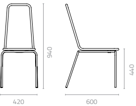
Olivia chair W420 x D600 x H940 x SH440mm Packing: 0.400m 3 , 4pcs/stack
